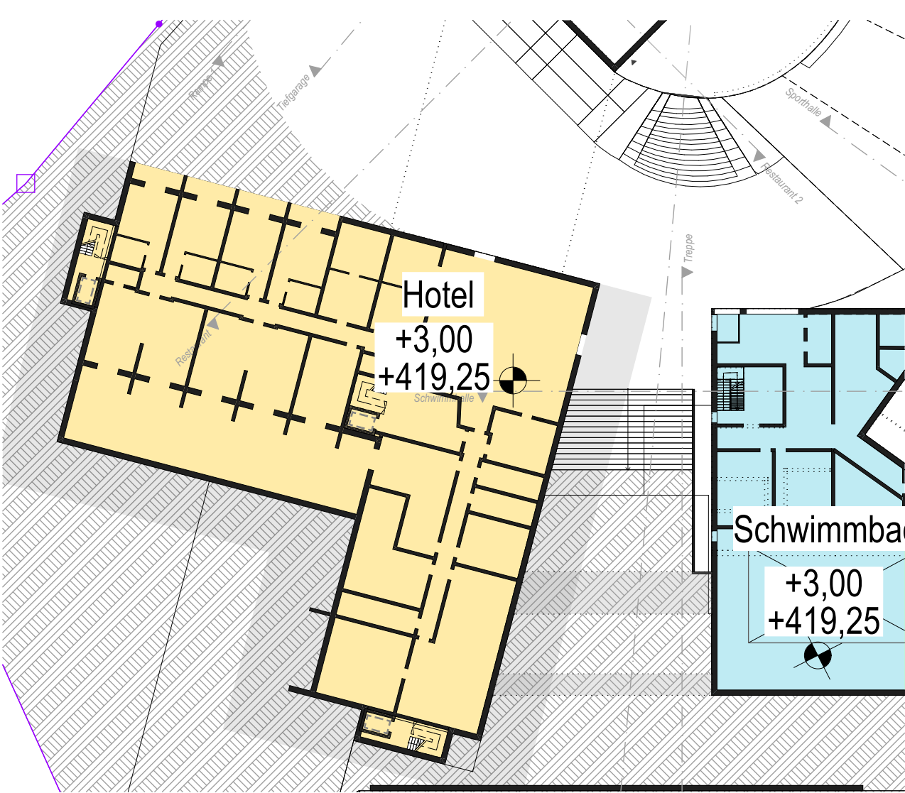
Hotel Erdgeschoss
